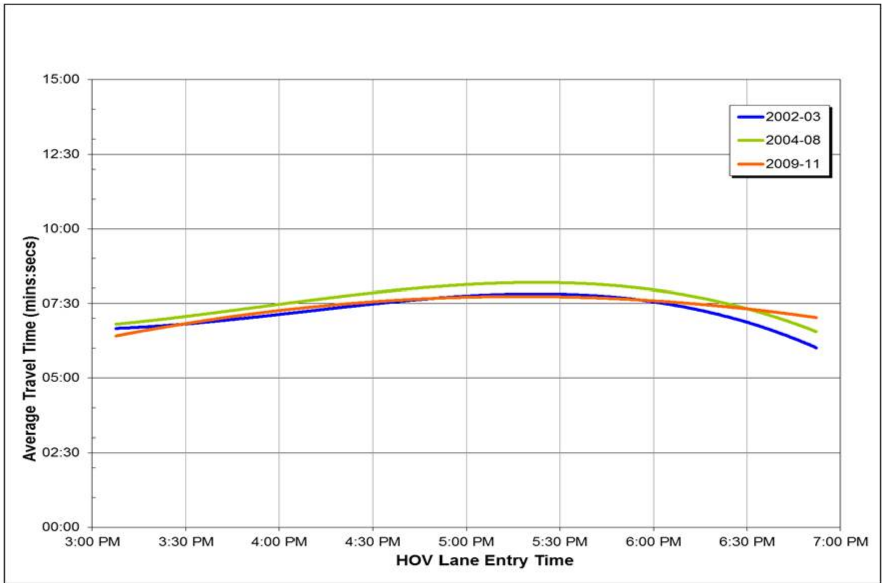
FIGURE 8 Southeast Expressway Travel Times: Southbound HOV Lane, PM Peak Period, 2002-11
